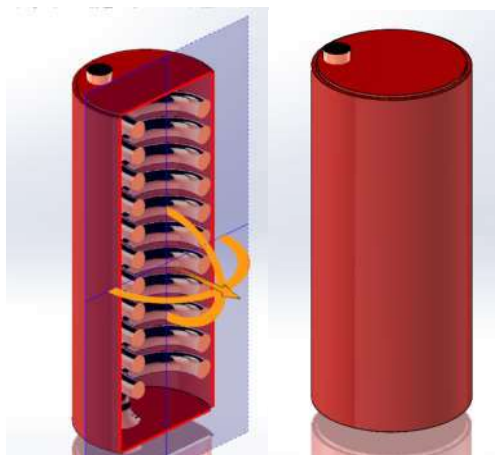
Figure 4. Evaporator Design
