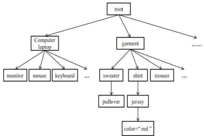
Fig. 3. An example of our extended concept hierarchy.
