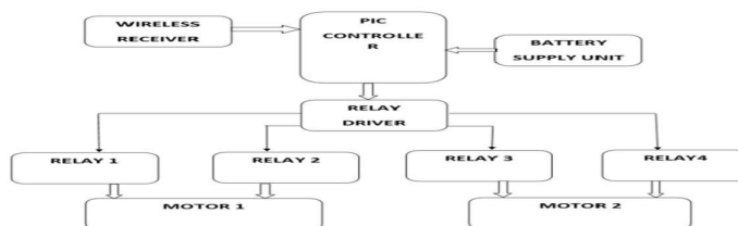
Fig 2: Block of receiver unit on wheelchair
