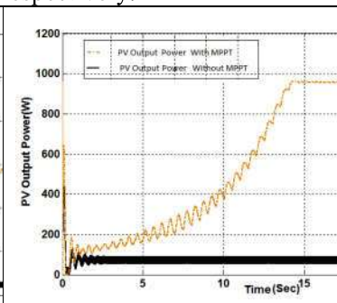
Figure 10 Output Power for the solar irradiance (600 w/m 2 ) in hybrid MPPT technique
