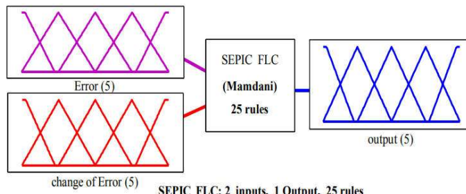
Figure 3. Membership function for MPP
