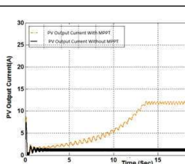
Figure 6 Output Current for the solar irradiance ( 500\text{ w/m}^2 ) in hybrid MPPT technique
