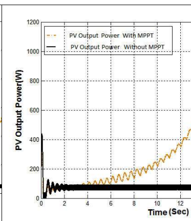
Figure 13 Output Power for the solar irradiance (1000 w/m 2 ) in hybrid MPPT technique
