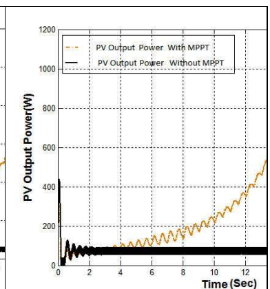
Figure 13 Output Power for the solar irradiance (1000 w/m 2 ) in hybrid MPPT technique
