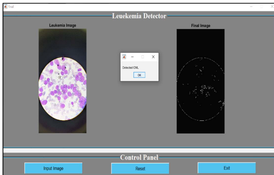
Fig.4. Detected CML
